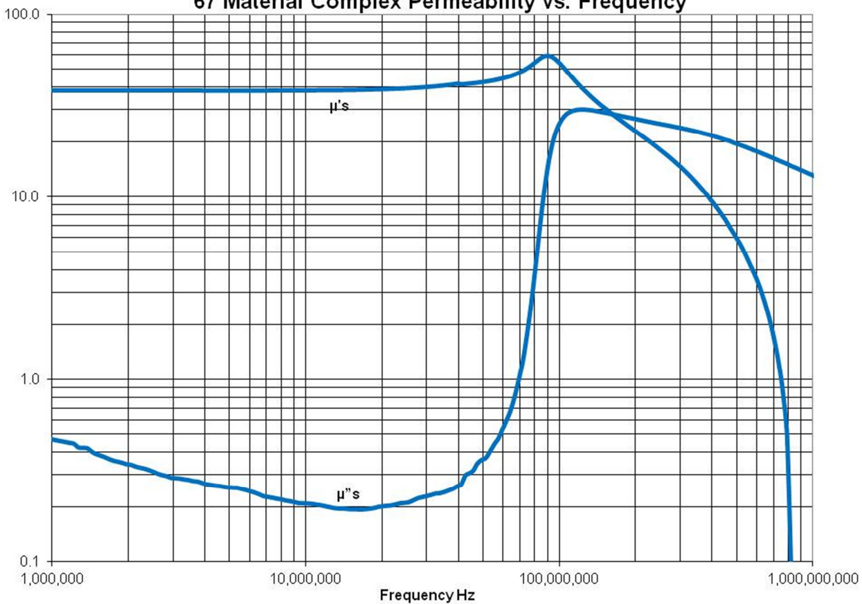
67 Material Complex Permeability vs. Frequency
