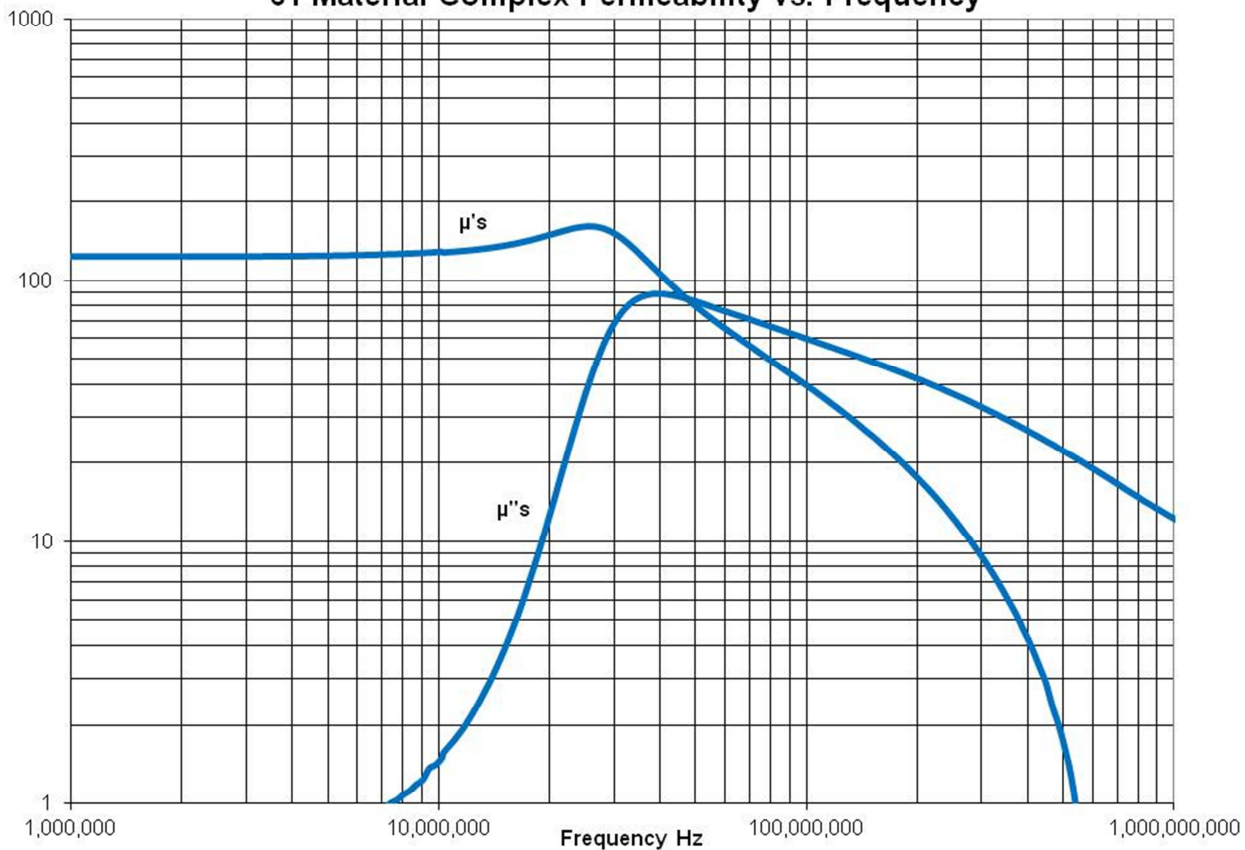
61 Material Complex Permeability vs. Frequency
